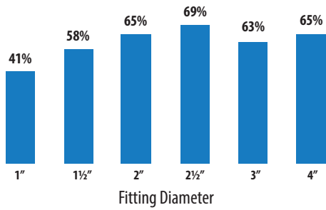
Average Head Loss Reduction: LASCO Sweep vs Standard 90° Elbow
